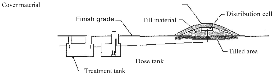
Figure 1 - A cross-section-of a mound system for POWTS.
