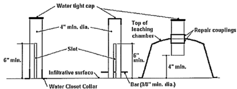
Figure 8 – Observation Pipes
