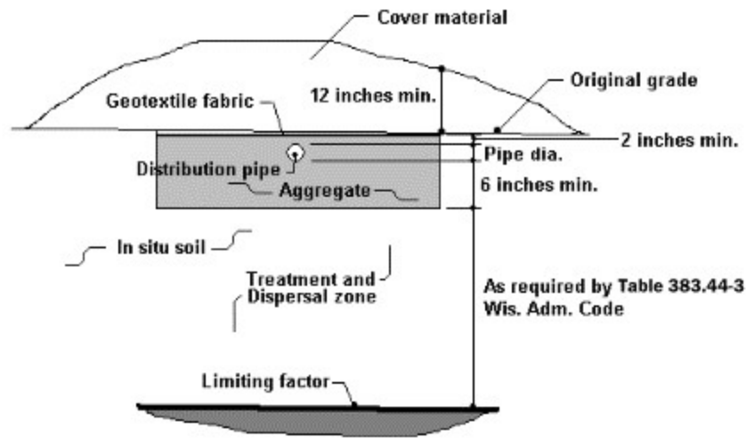
Figure 3 - Height of system when using aggregate.
