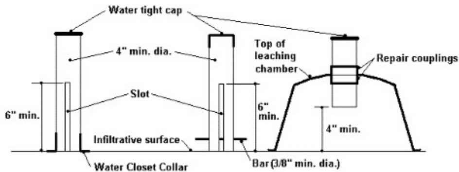
Figure 5 - Observation pipes
